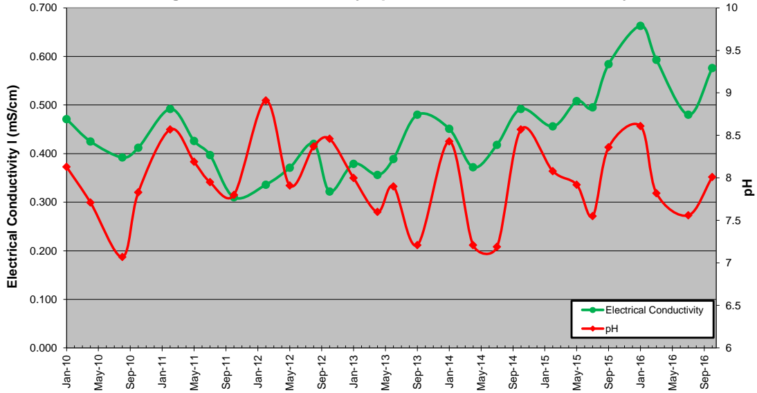
Cudgen Lakes Sand Quarry - pH and Electrical Conductivity
